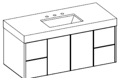
48" version
